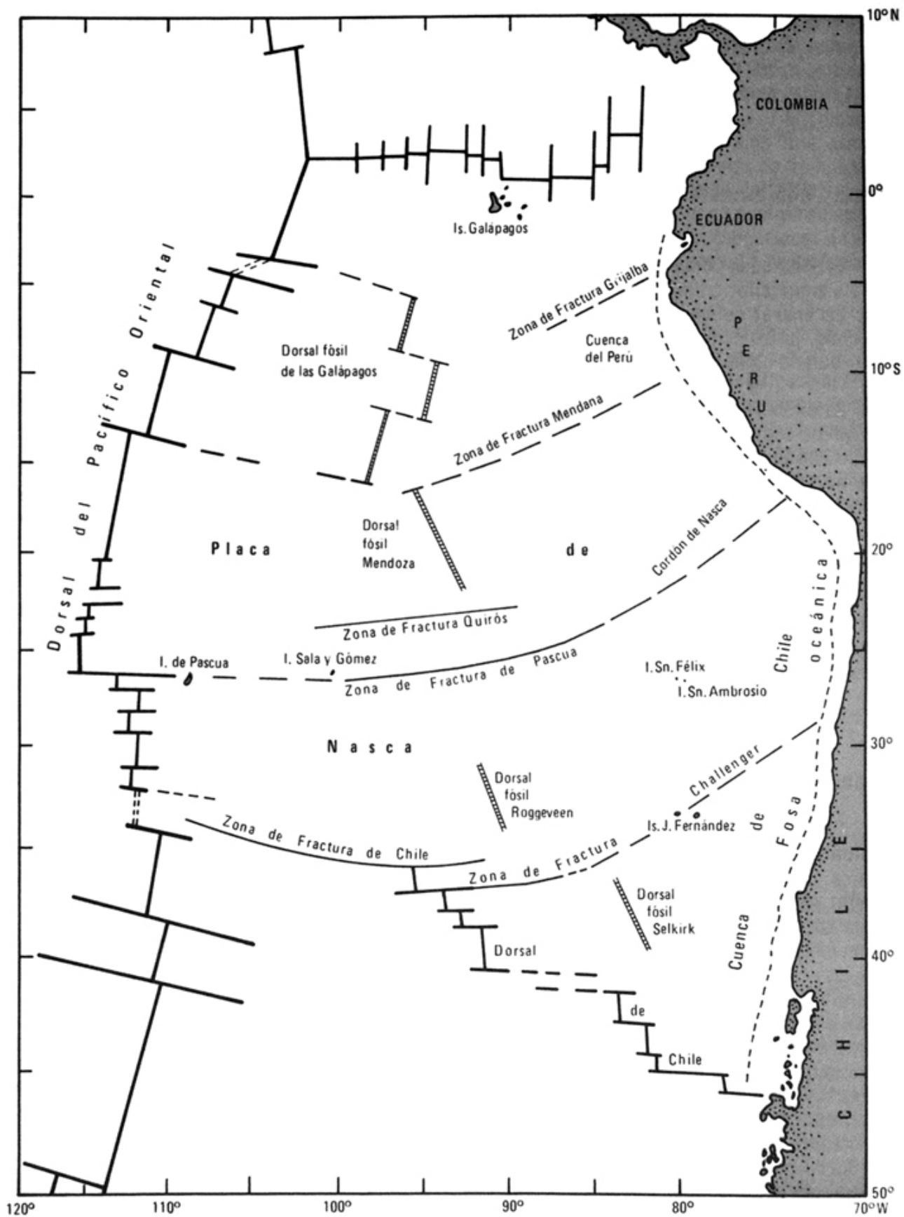
OCEANO PACIFICO SURORIENTAL. RELIEVE SUBMARINO
